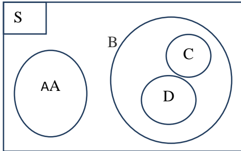
Gambar 4. Diagram Venn
